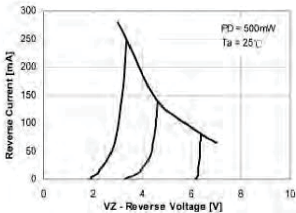
Figure 5. Reverse Current vs. Reverse Voltage
