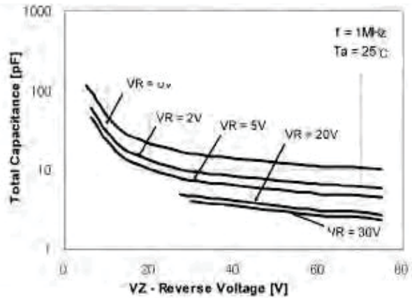
Figure 2. Total Capacitance
