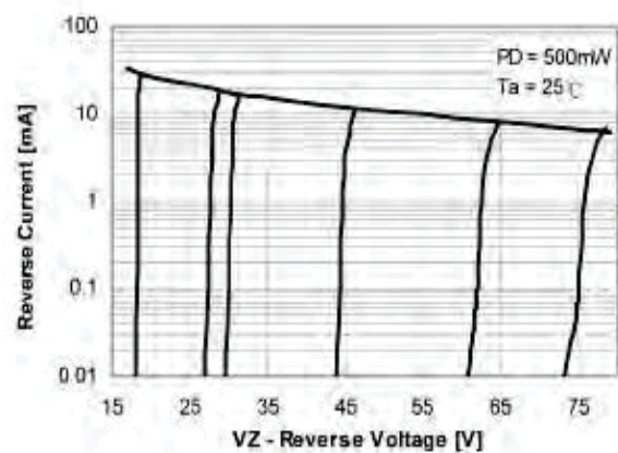
Figure 6. Reverse Current vs. Reverse Voltage
